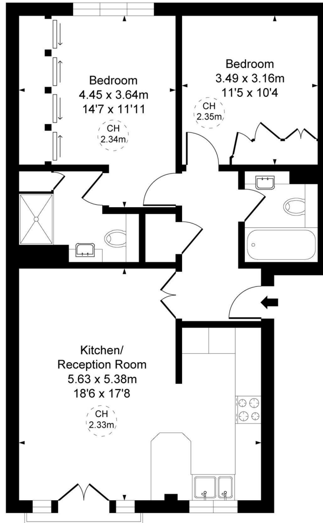
Fourth Floor
